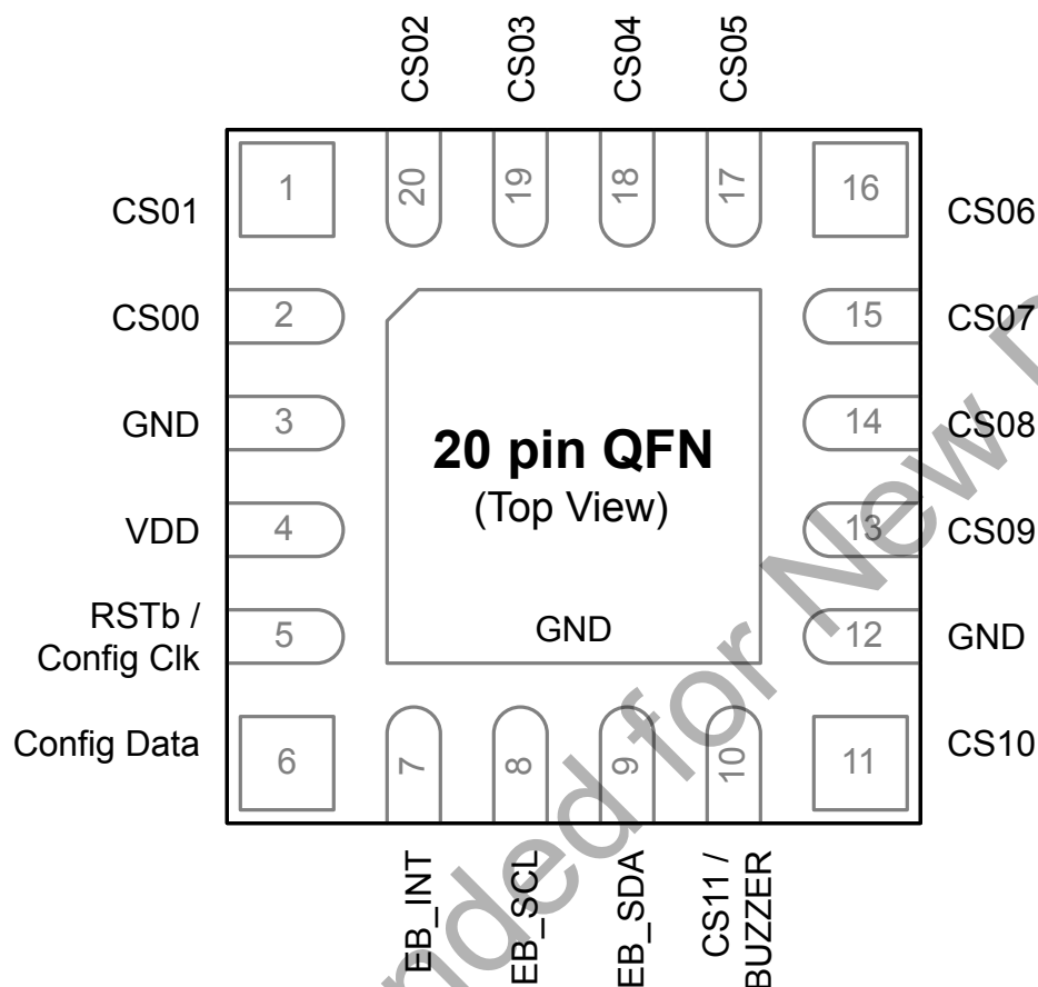
Figure 5.1. CPT212B QFN20 Pinout
